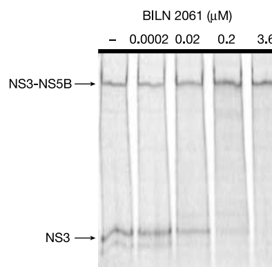
Figure 2 BILN 2061 inhibition of HCV polyprotein processing. Inhibition of NS3-protease-mediated polyprotein processing in cells containing an HCV 1b subgenomic NS2-NS5B replicon. To detect HCV non-structural protein precursors and NS3 mature protein, replicon-containing cells treated with increasing amounts of BILN 2061 were pulse-labelled for 2 h with 35 S-labelled methionine/cysteine. After incubation, cell extracts were immunoprecipitated with a specific anti-NS3 protein antibody and products were analysed by SDS–PAGE followed by phosphor imaging as previously described 18 . The position of the NS3-NS5B precursor and the NS3 mature protein are indicated.
