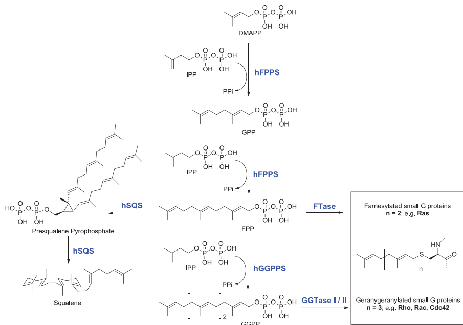
FIGURE 2 | Structures and sequence of steps involved in the biosynthesis of key isoprenoids.
