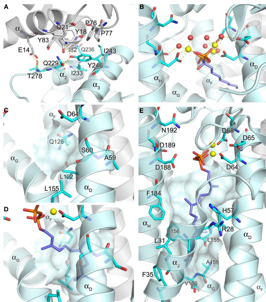
FIGURE 5 | Structure of geranylgeranyl pyrophosphate synthase.
