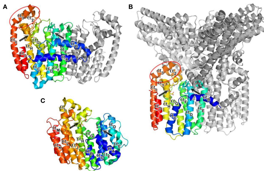
FIGURE 3 | Overall structures of human prenyl synthase enzymes.
