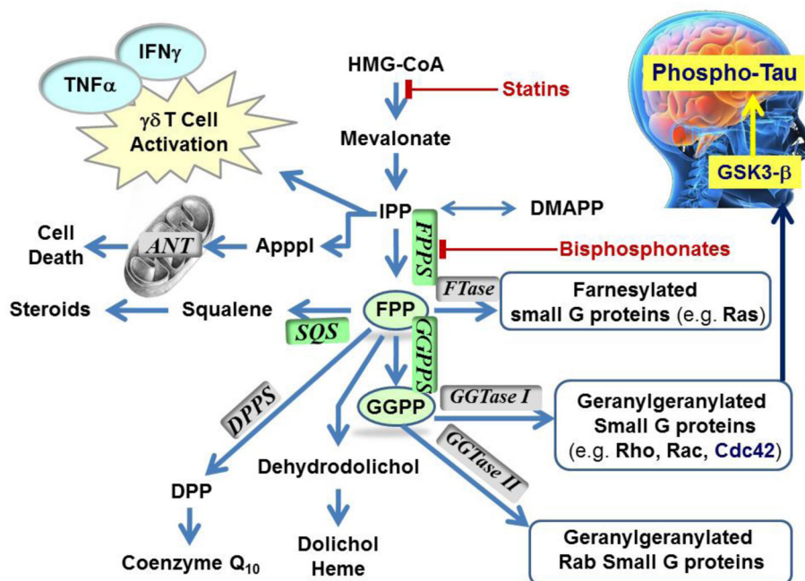
FIGURE 1 | Schematic representation of the mevalonate pathway, indicating the major biochemical effects of isoprenoids. Classes of current drugs that modulate the function of key enzymes include Statins and
